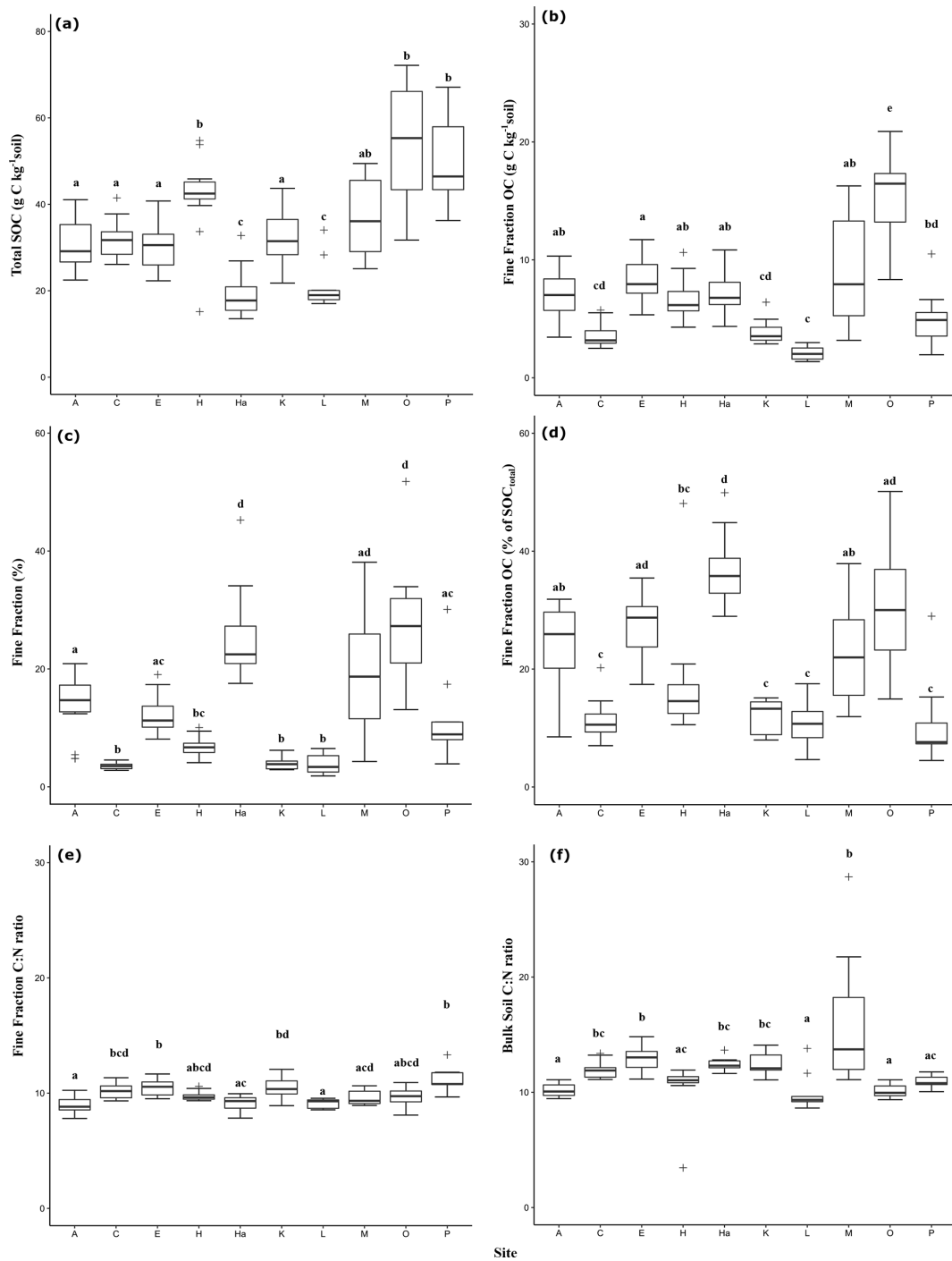
Figure 1. Measured total SOC (g C per kg soil) (a), total fine-fraction organic carbon (g C per kg soil) (b), mass proportion of the fine fraction (< 20 \mu\text{m} , %) (c), relative proportion of measured fine-fraction organic carbon of the total SOC content of the bulk soil (d), fine-fraction C : N ratio (e) and bulk-soil C : N ratio (f) for each of the grassland sites: Aberystwyth (A), Crichton (C), Easter Bush (E), Hillsborough (H), Harpenden (Ha), Kirkton (K), Llangorse (L), Myerscough (M), Overton (O) and Plumpton (P). Boxes represent the 25th and 75th percentile, with lines showing the median value. Whiskers show the lowest and highest values with outliers indicated as crosses (> 1.5 times the interquartile range). Lettering indicates significant differences between soils ( p < 0.05 ).
