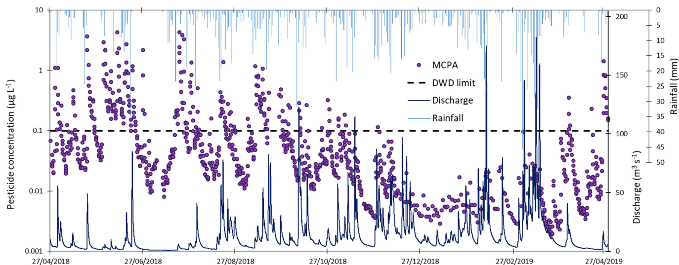
Fig. 3. Concentration of MCPA in the River Derg at the catchment outlet and abstraction point, the River Derg discharge 7 km upstream of the monitoring point at Castlederg, and Malin Head daily rainfall between 27/04/18 and 30/04/19. The single pesticide drinking water limit for treated water is shown for reference as a dashed line. Note that the pesticide concentrations are shown on a log scale on the left y-axis.
